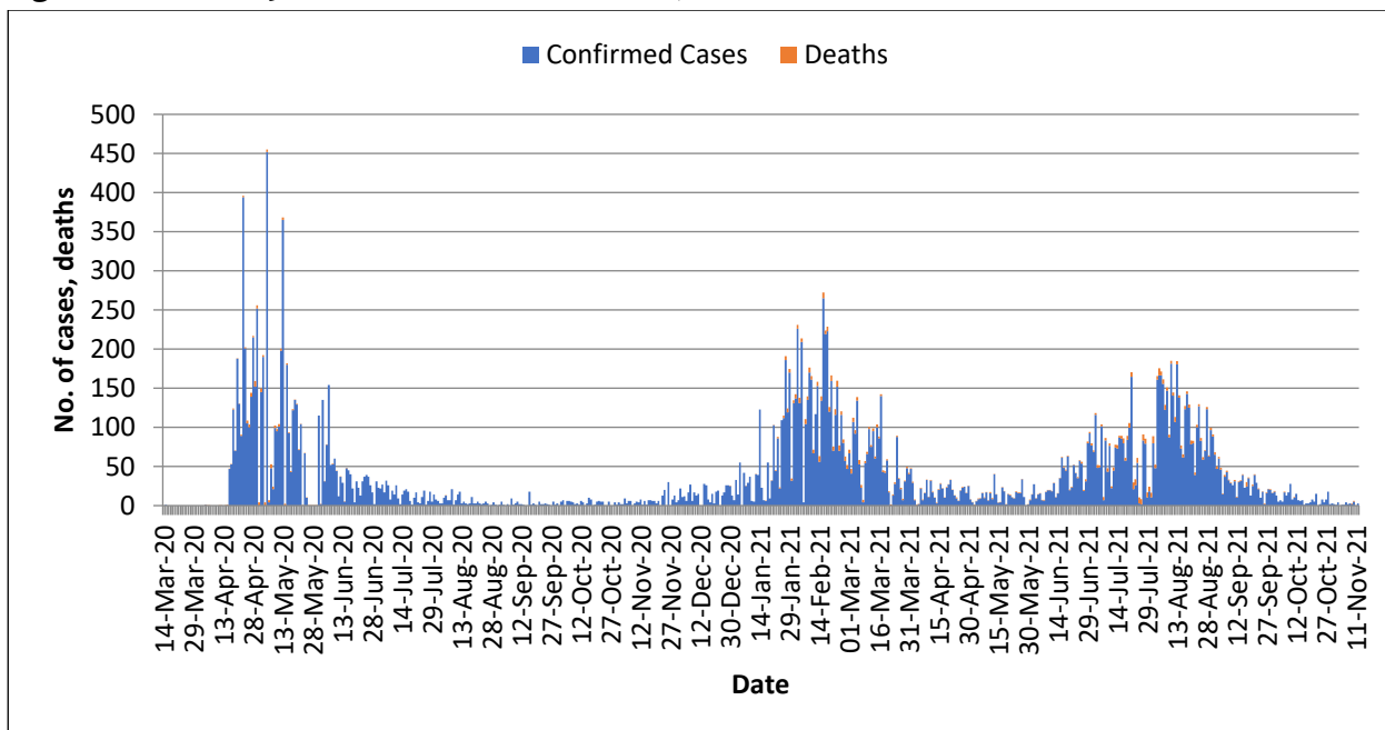
Figure 2: COVID – 19 confirmed cases and deaths, 06 to 12 November 2021 Tanzania Mainland
